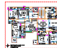
1ST-4TH FLOOR PLAN
